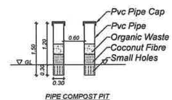
PIPE COMPOST PIT
