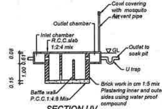
SECTION UV
