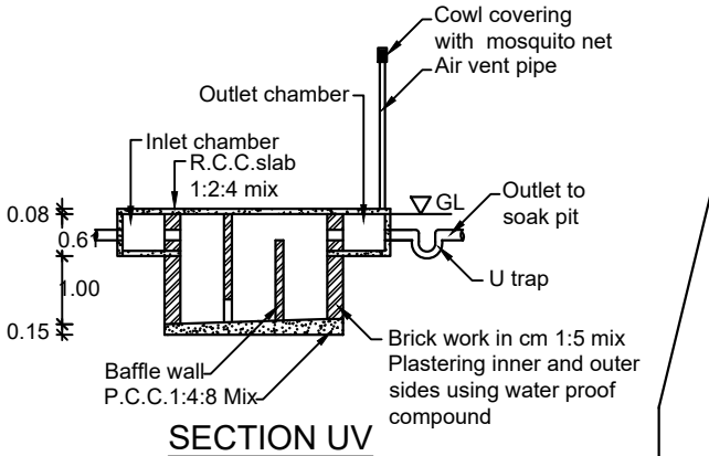
SECTION UV
