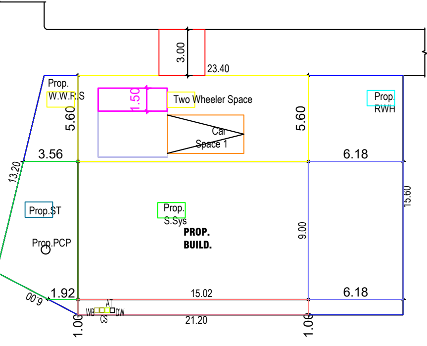
SITE PLAN
