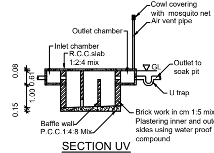
SECTION UV
