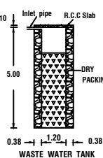
WASTE WATER TANK
