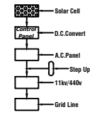
Solar System Flow Diagram
