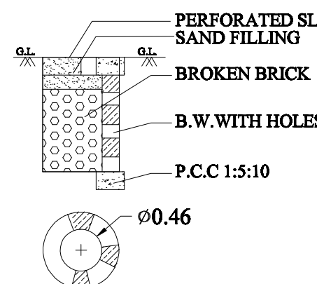
RAIN WATER PERCOLATION DRAWING TYPE -1A
