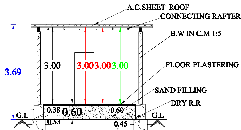
SECTION-AB
