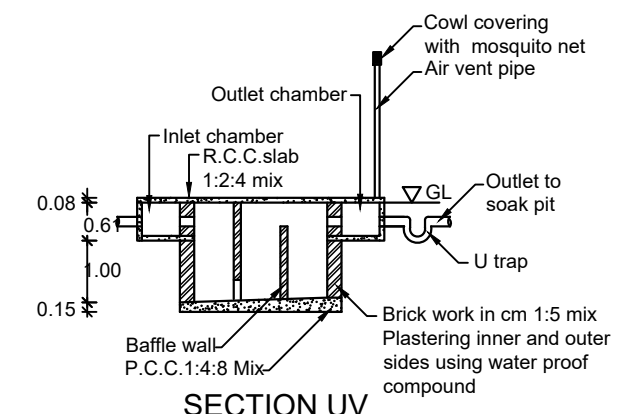
SECTION UV
