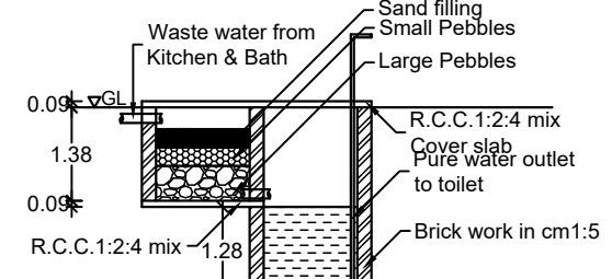
WASTE WATER RECYCLING SYSTEM
