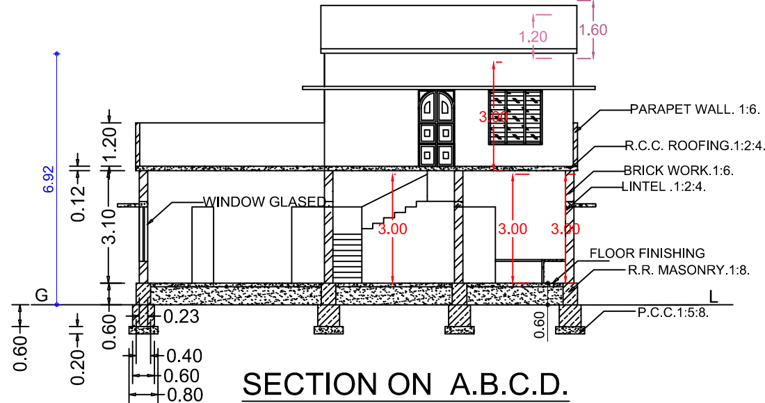
SECTION ON A.B.C.D.
