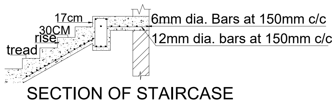
SECTION OF STAIRCASE
