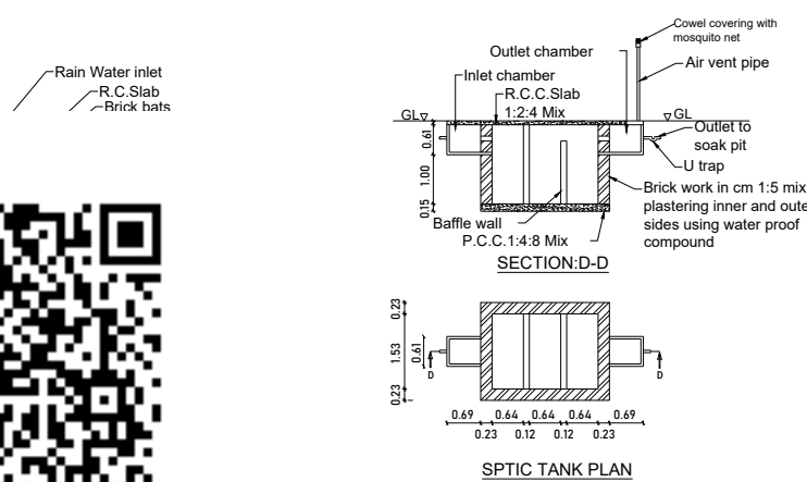
SPTIC TANK PLAN
