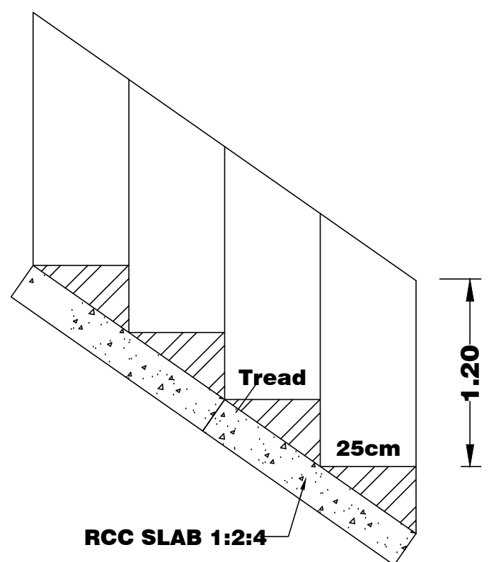
STAIR DETAILS
