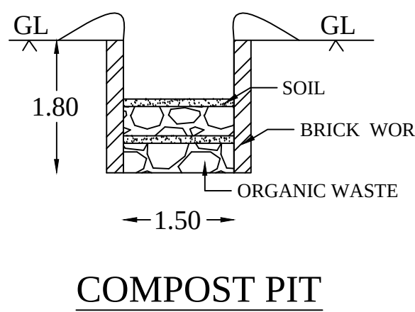
COMPOST PIT
