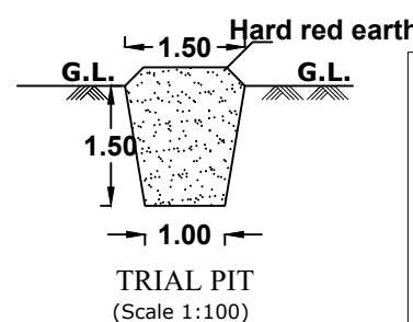
TRIAL PIT
