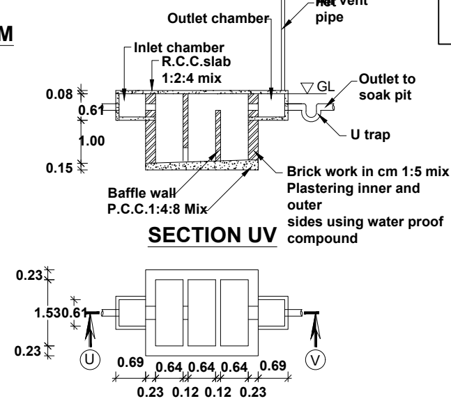
SEPTIC TANK PLAN
