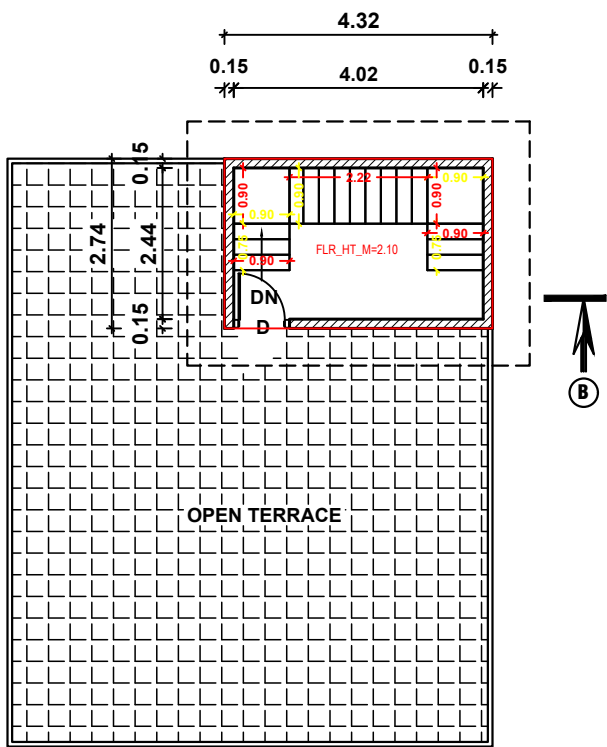
HEAD ROOM PLAN
