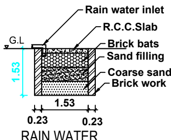
RAIN WATER HARVESTING PIT RWH_CAPACITY_L=5000LTRS
