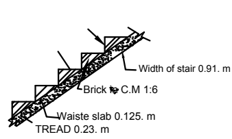
Stair Details
