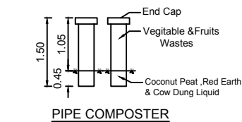
PIPE COMPOSTER
