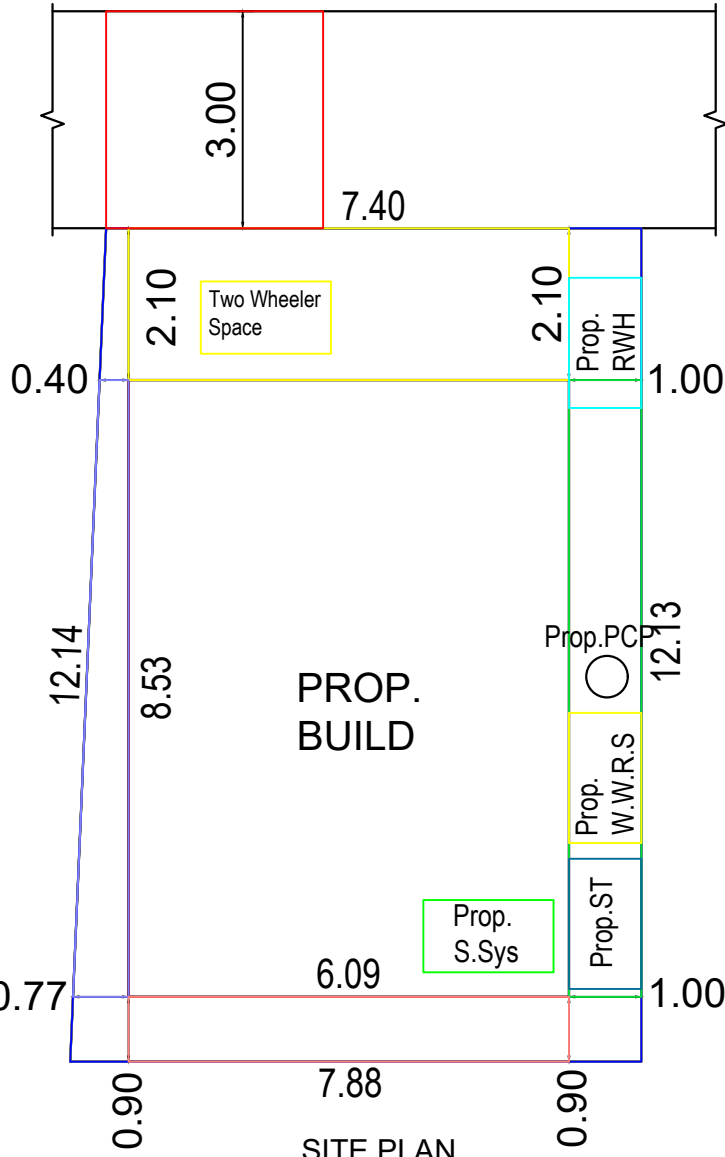
SITE PLAN
