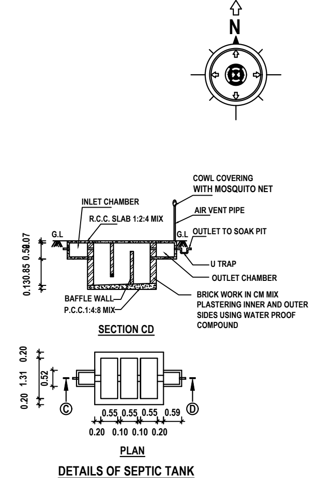
DETAILS OF SEPTIC TANK
