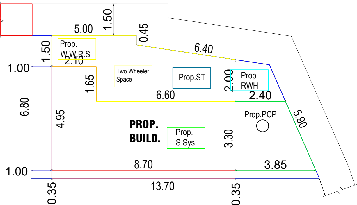
SITE PLAN
