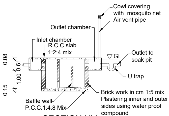
SECTION UV
