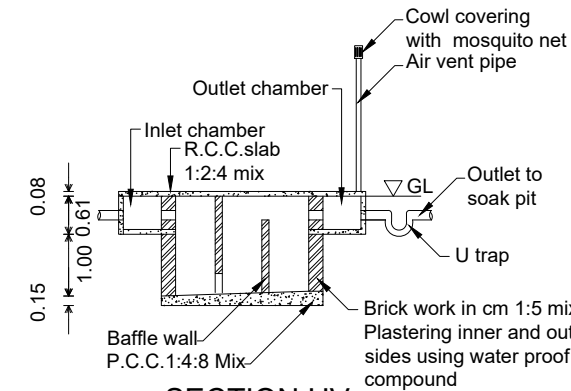
SECTION UV
