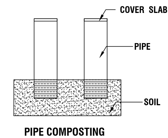
PIPE COMPOSTING
