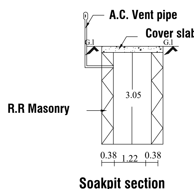
Soakpit section
