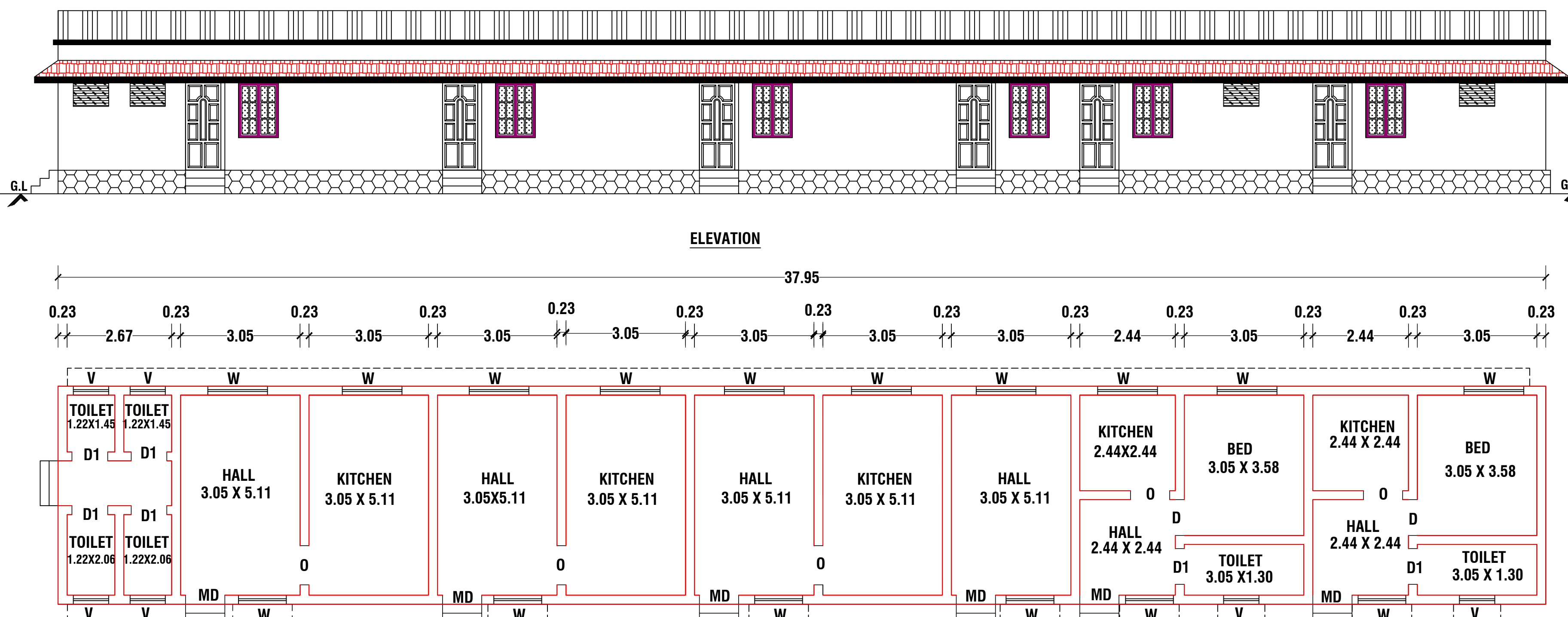
GROUND FLOOR PLAN SCALE 1:100 ALL DIMENSIONS ARE IN "METER"
