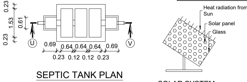
SOLAR SYSTEM
