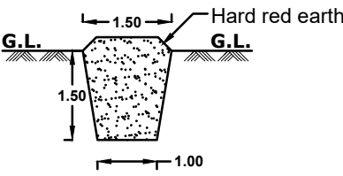
TRIAL PIT (Scale 1:100)
