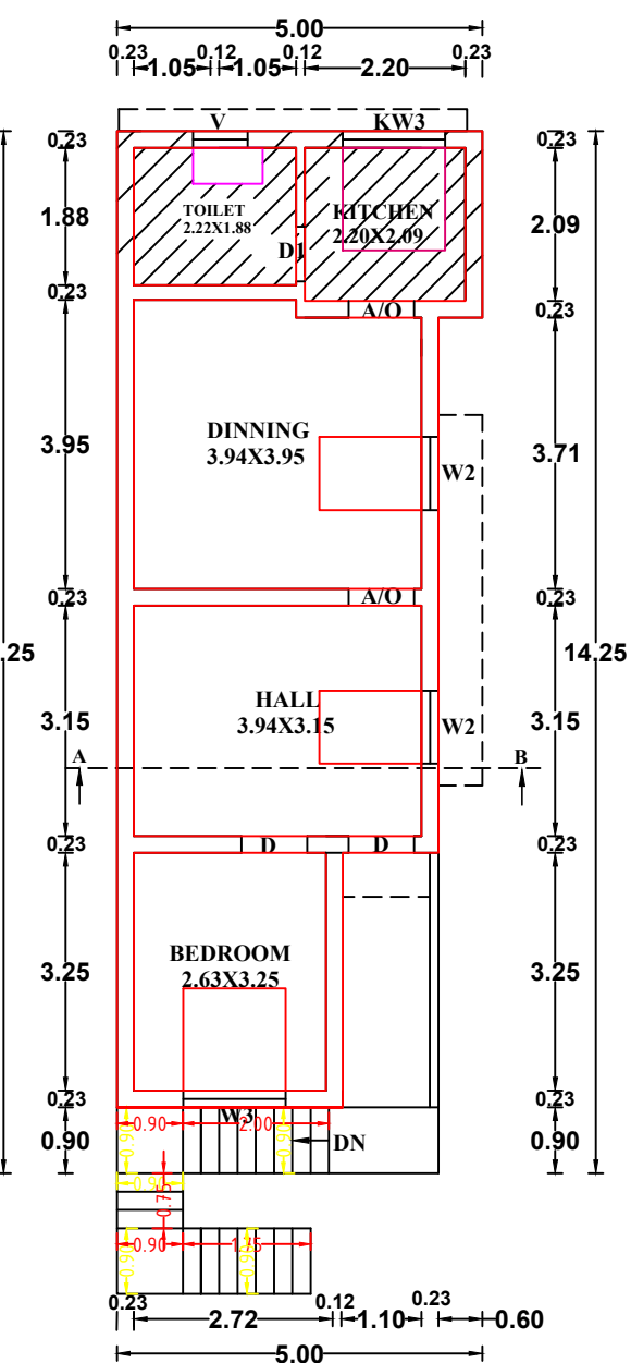
EXISTING FIRST FLOOR PLAN PROPOSED FIRST FLOOR PLAN
