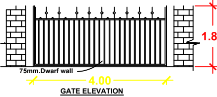
GATE ELEVATION
