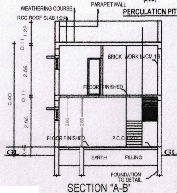
SECTION "A-B"
