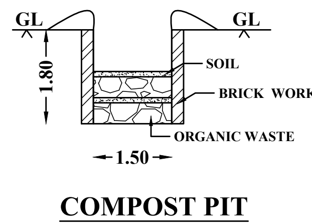
COMPOST PIT
