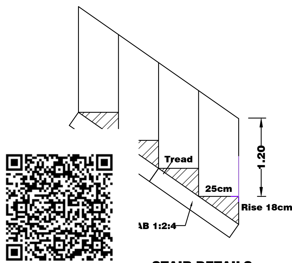
STAIR DETAILS
