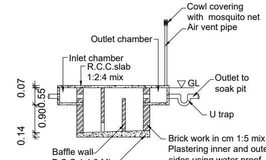
SECTION UV
