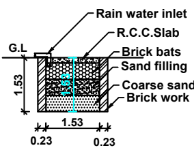
RAIN WATER HARVESTING PIT RWHT CAPACITY_L=5000LTRS
