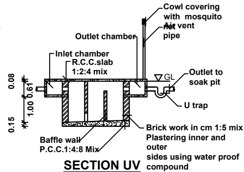
SECTION UV
