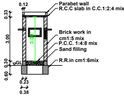
SECTION ON ST
