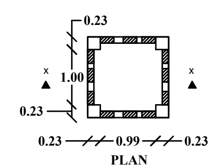
RAIN WATER HARVEST WELL
