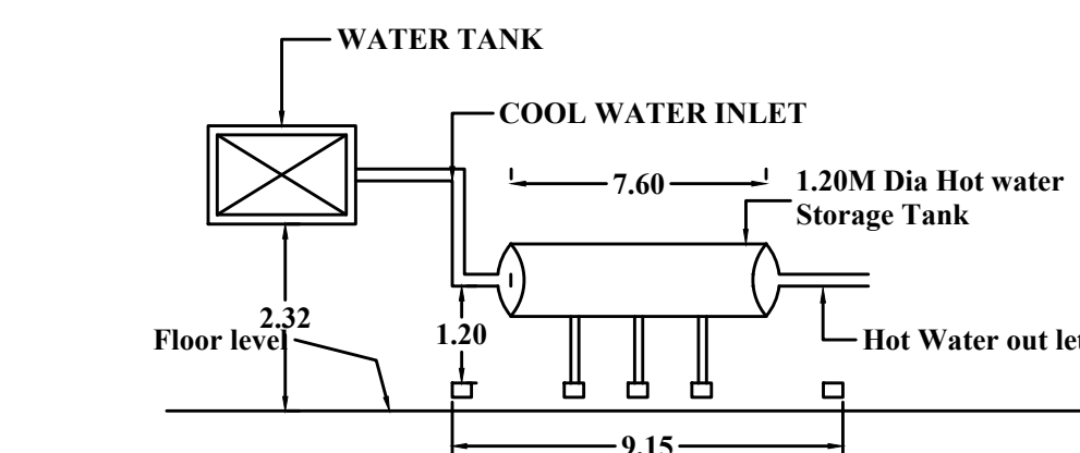
SOLAR WATER HEATING SYSTEM( S.W.H.S.DETAILS)
