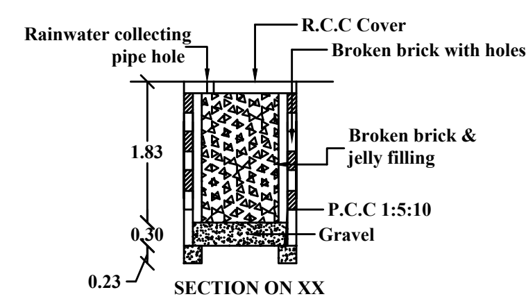
SECTION ON XM
