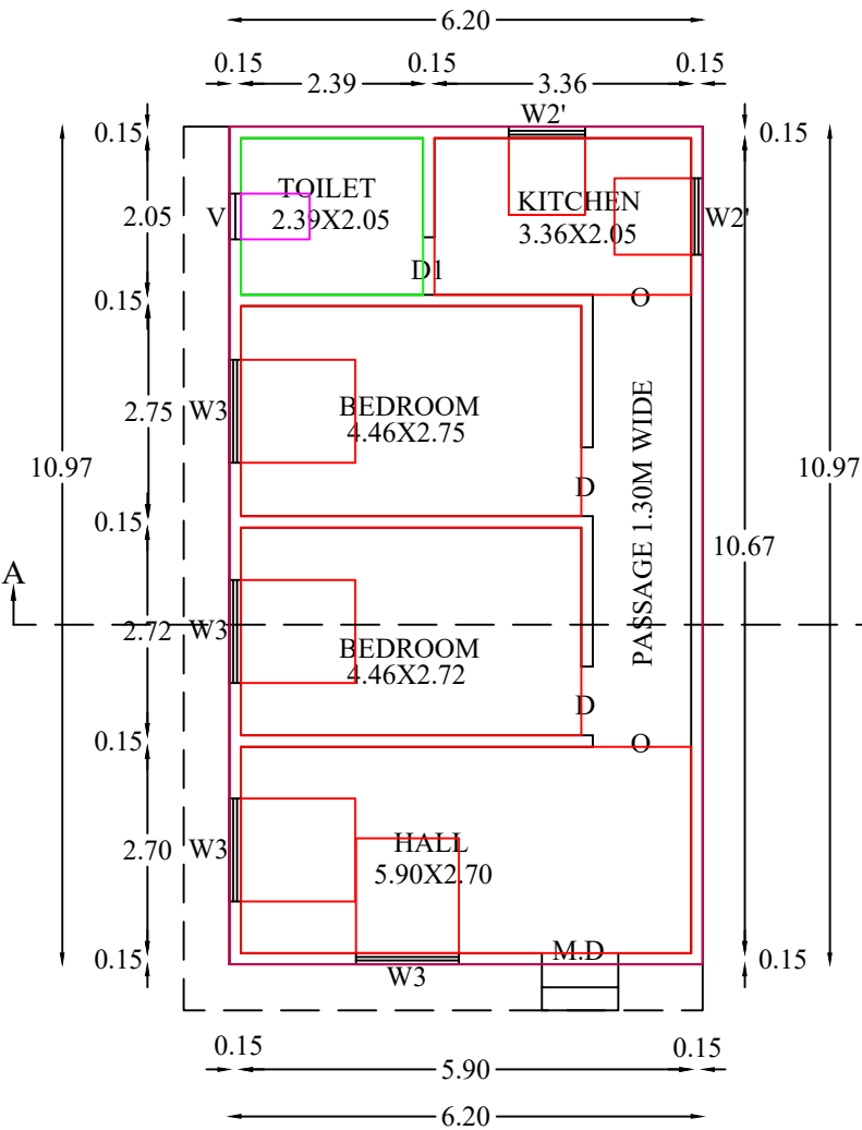
PLAN
