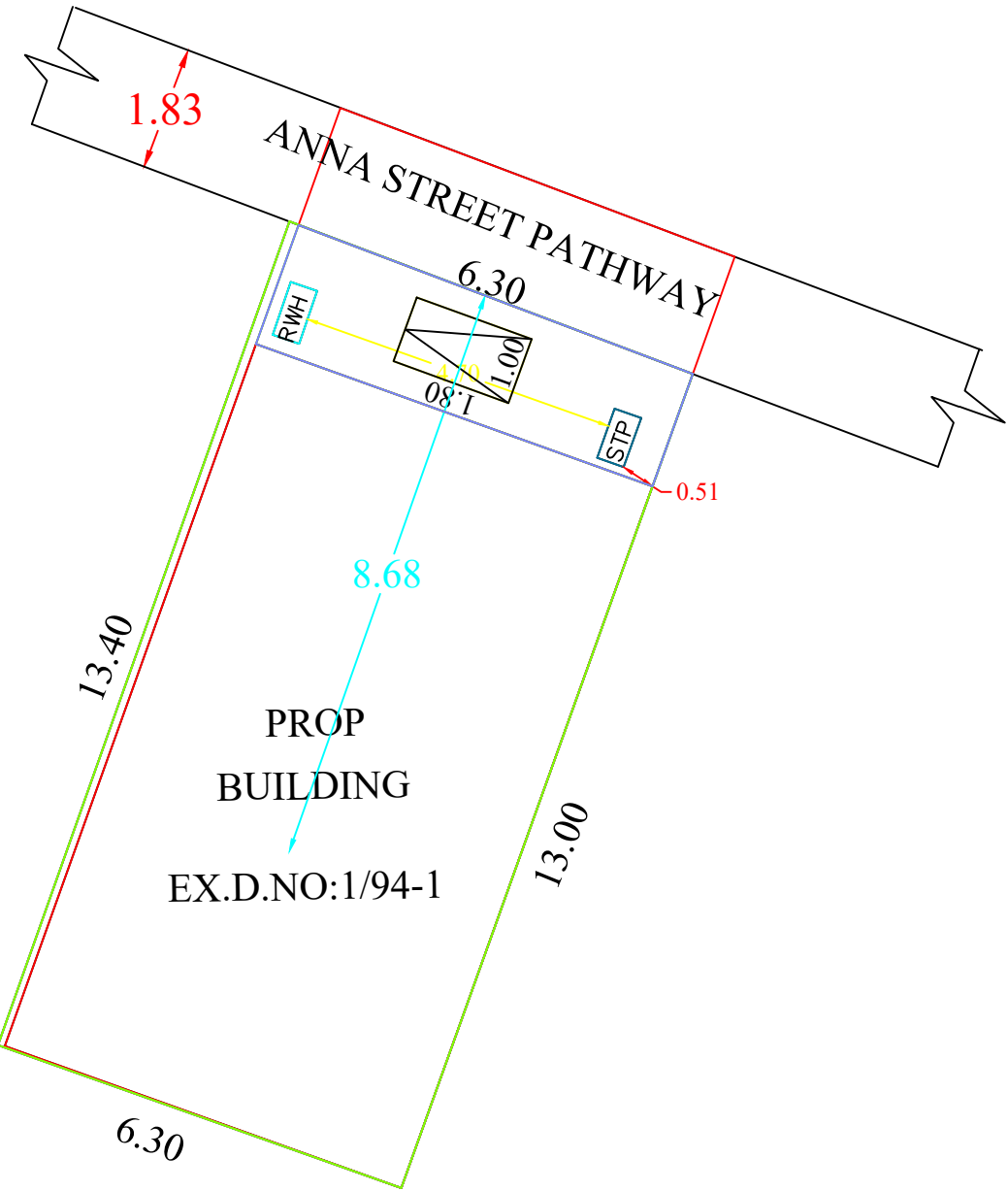
SITE PLAN
