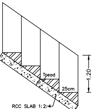
STAIR DETAILS
