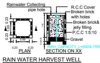
RAIN WATER HARVEST WELL
