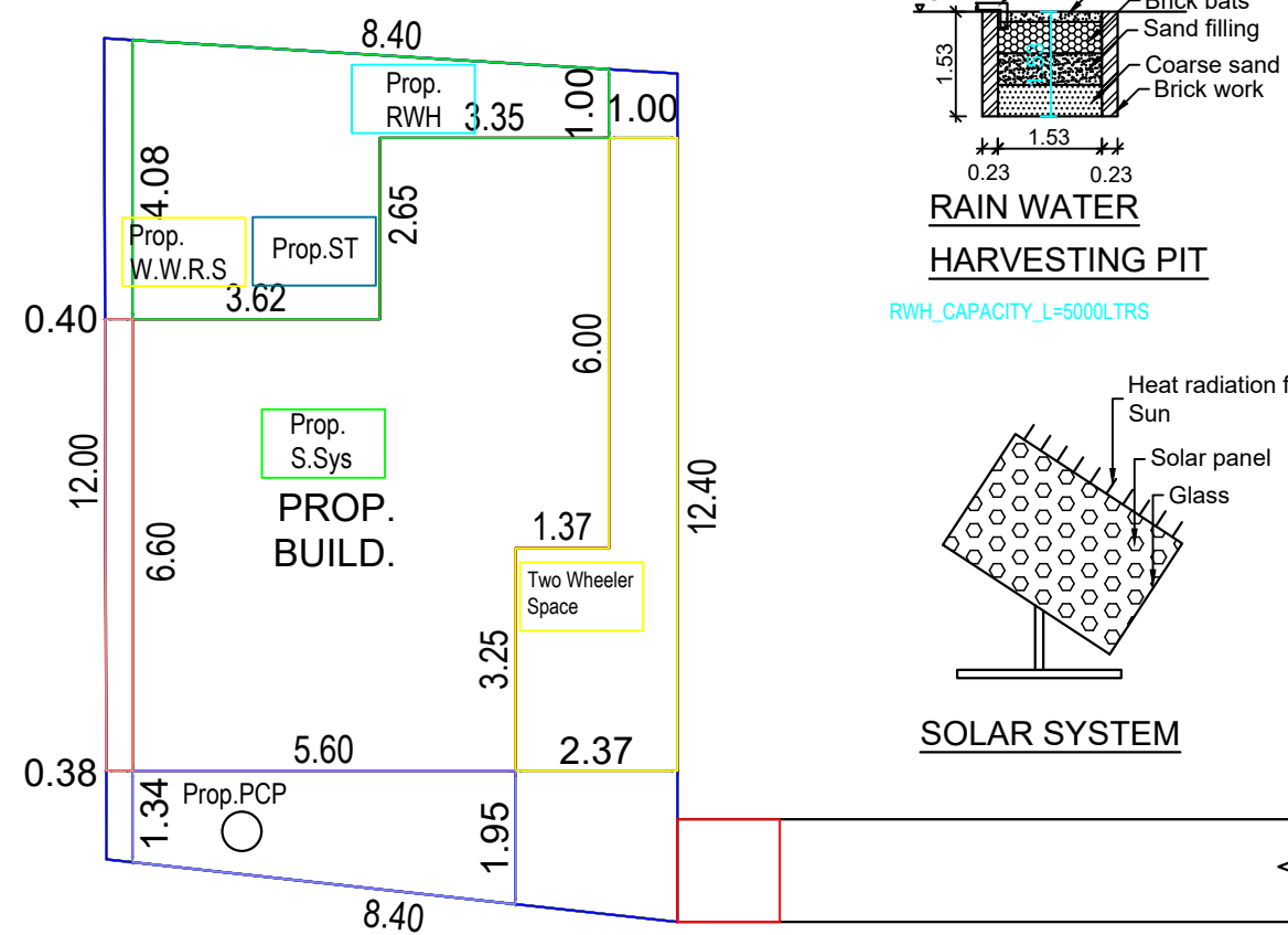
SITE PLAN
