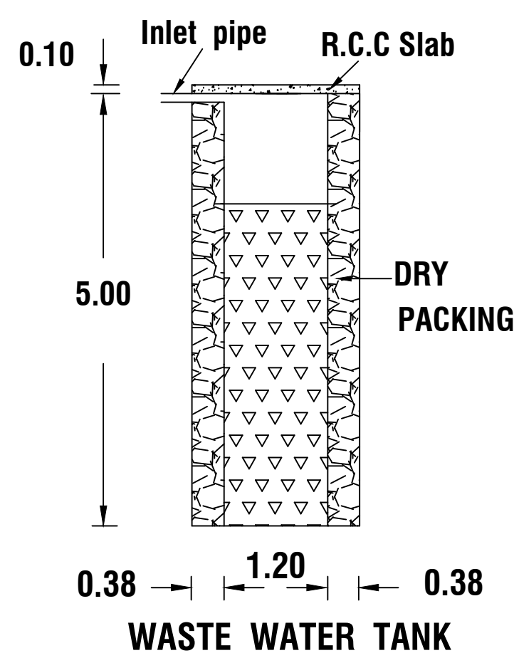
WASTE WATER TANK
