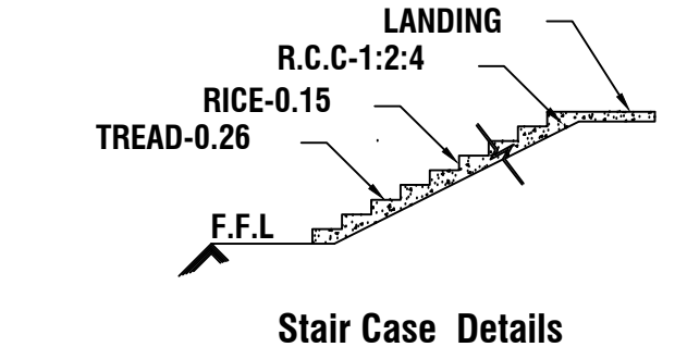
Stair Case Details
