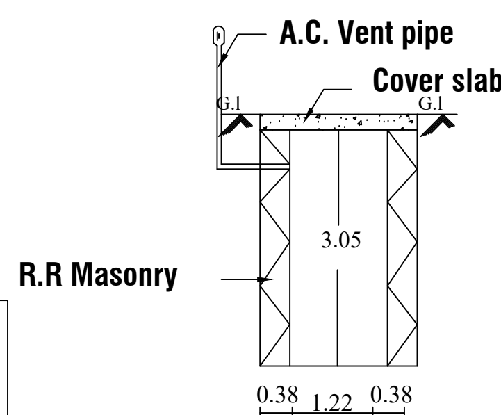
Soakpit section
