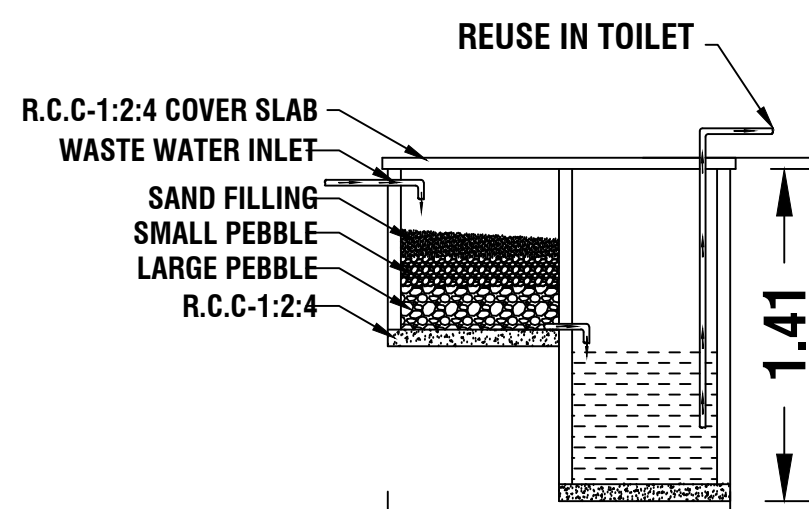
RECYCLING OF WASTE WATER
