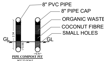
PIPE COMPOST PIT NOT TO SCALE
