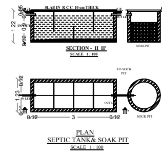
PLAN SEPTIC TANK & SOAK PIT SCALE 1:100
