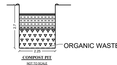
COMPOST PIT NOT TO SCALE
