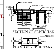
RECYCLING OF WASTE WATER KITCHEN & BATH ROOM
