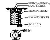
RAIN WATER PERCOLATION DRAWING TYPE -1A
