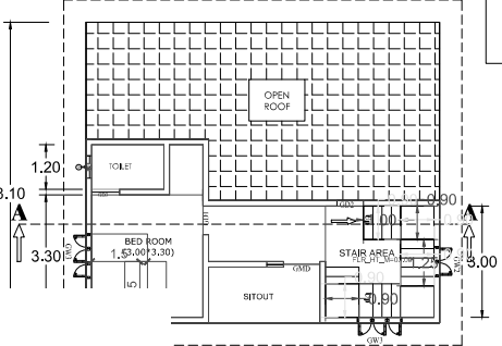
T FLOOR - PLAN
