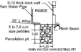
RAIN WATER HARVESTING PIT
