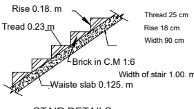
STAIR DETAILS
