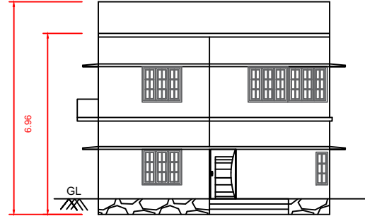
ELEVATION [1:100]
