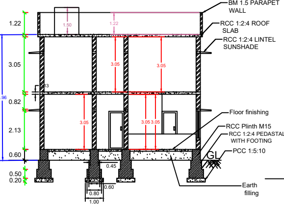
SECTION ON A-B [1:100]
