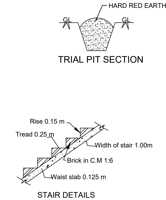
STAIR DETAILS
