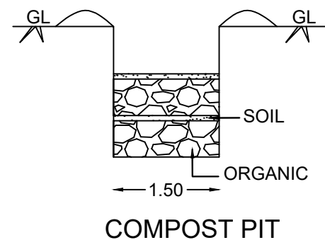
COMPOST PIT
