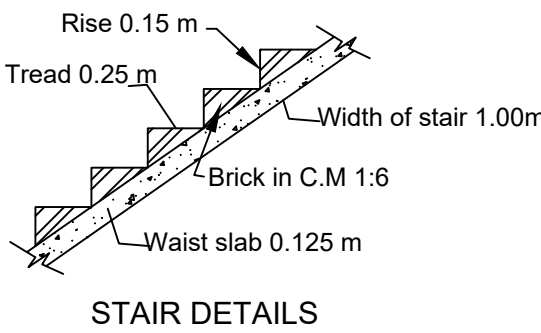
STAIR DETAILS
