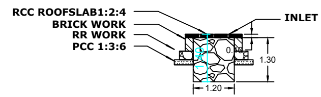
RAIN WATER HARVEST TRENCH
