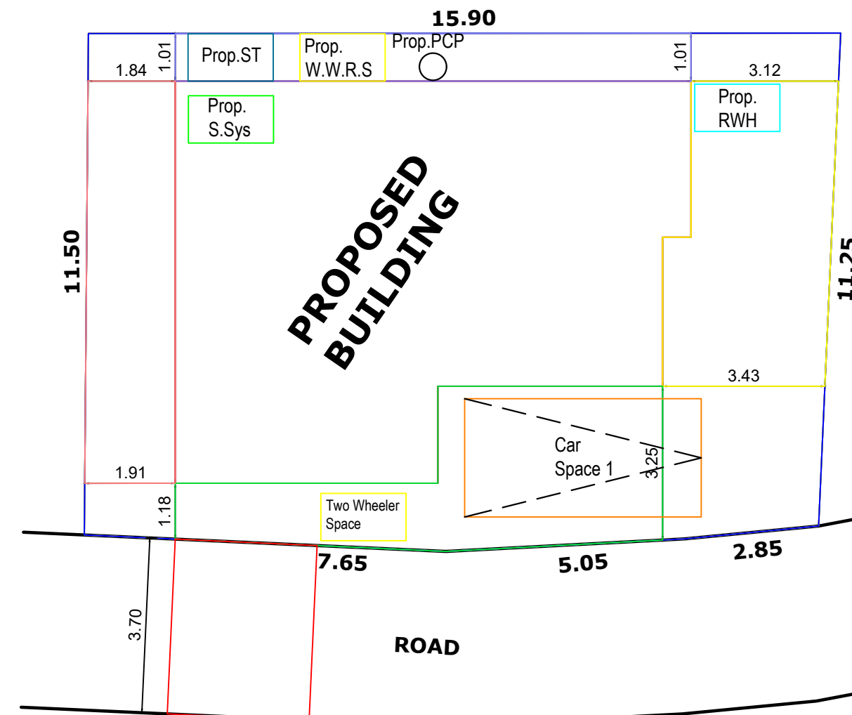
SITE PLAN
