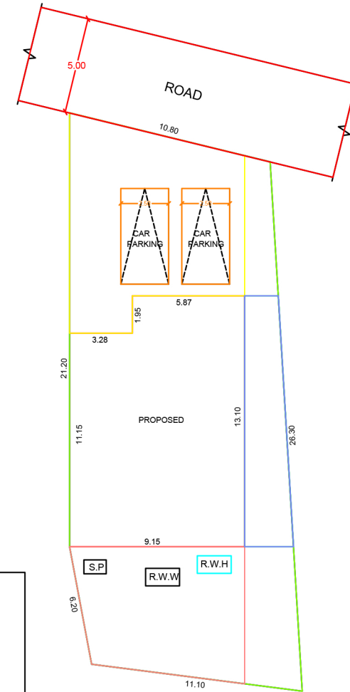
SITE PLAN SCALE:1:100
