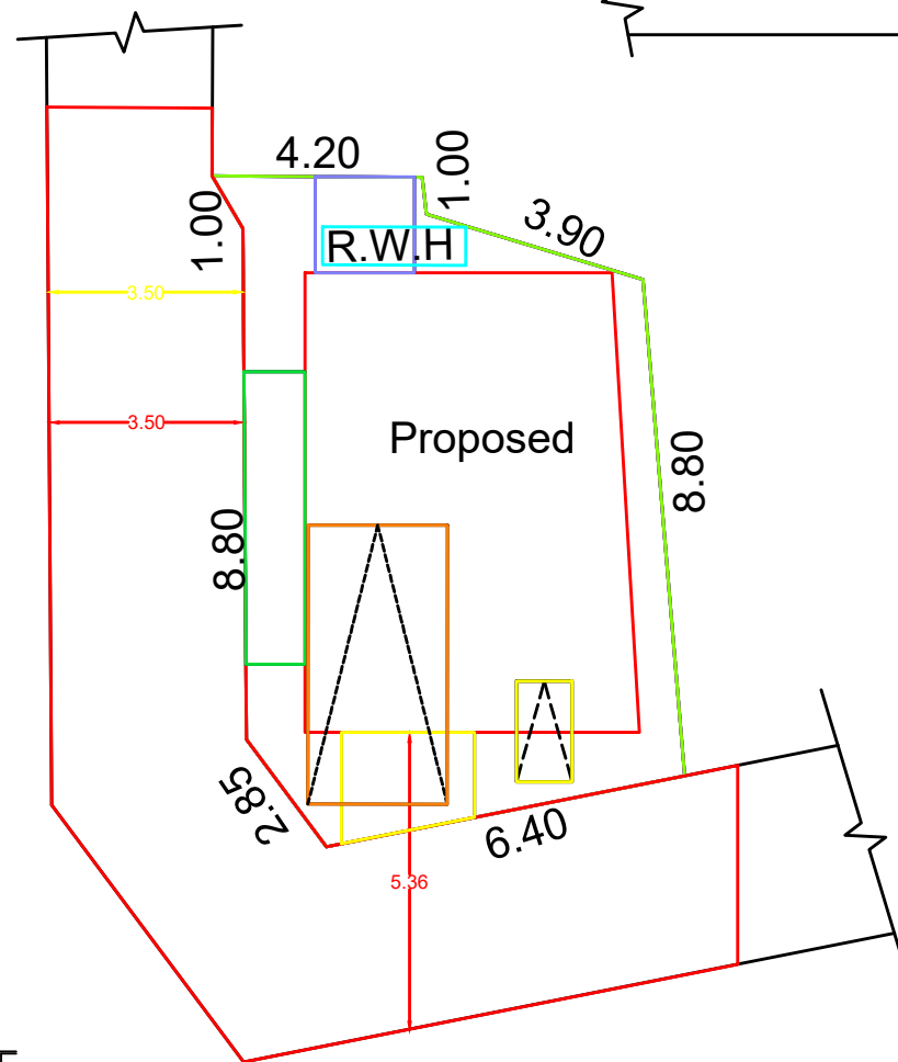
SITE PLAN
