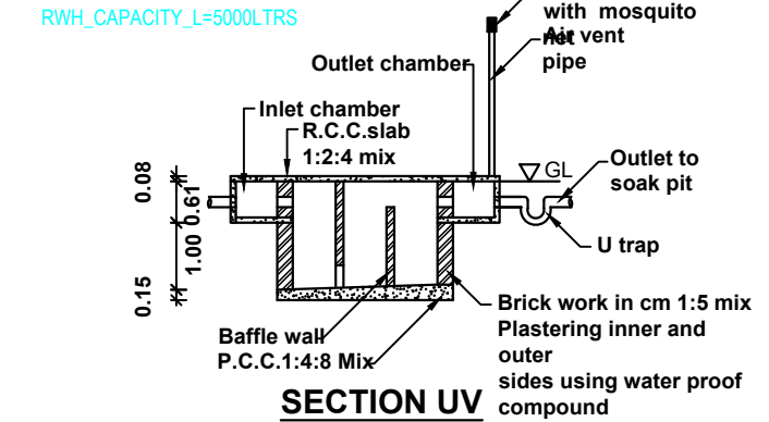
SECTION UV
