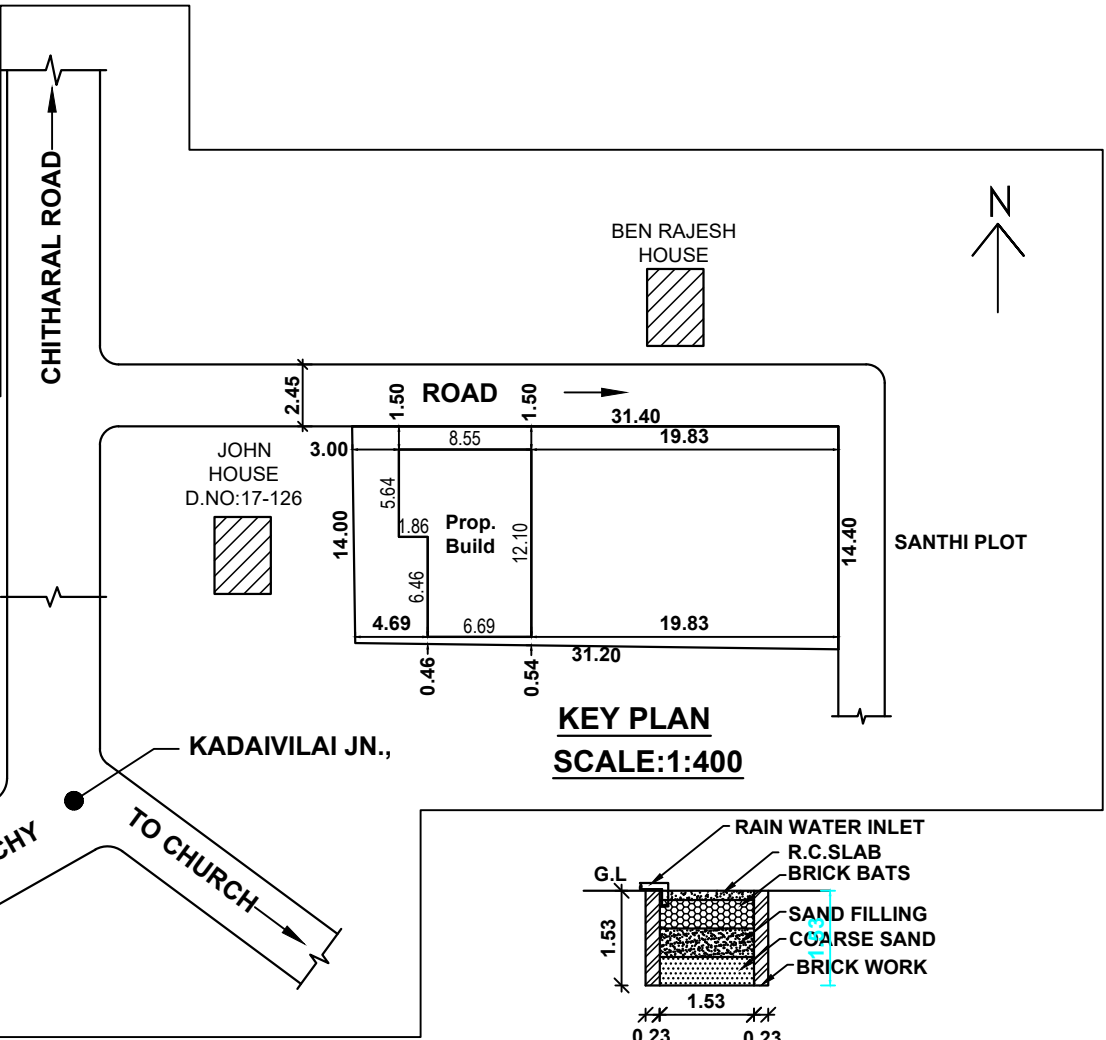
RAIN WATER HARVESTING TANK
