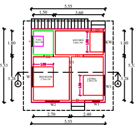
GROUND FLOOR PLAN AREA:30.69M2(330.22SQ.FT)
