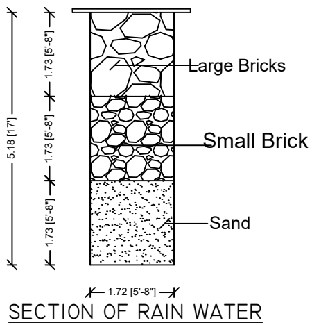
SECTION OF RAIN WATER
