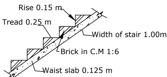
STAIR DETAILS
