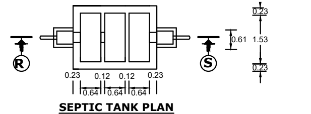
SEPTIC TANK PLAN
