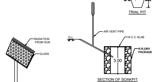
SECTION OF SOAKPIT
