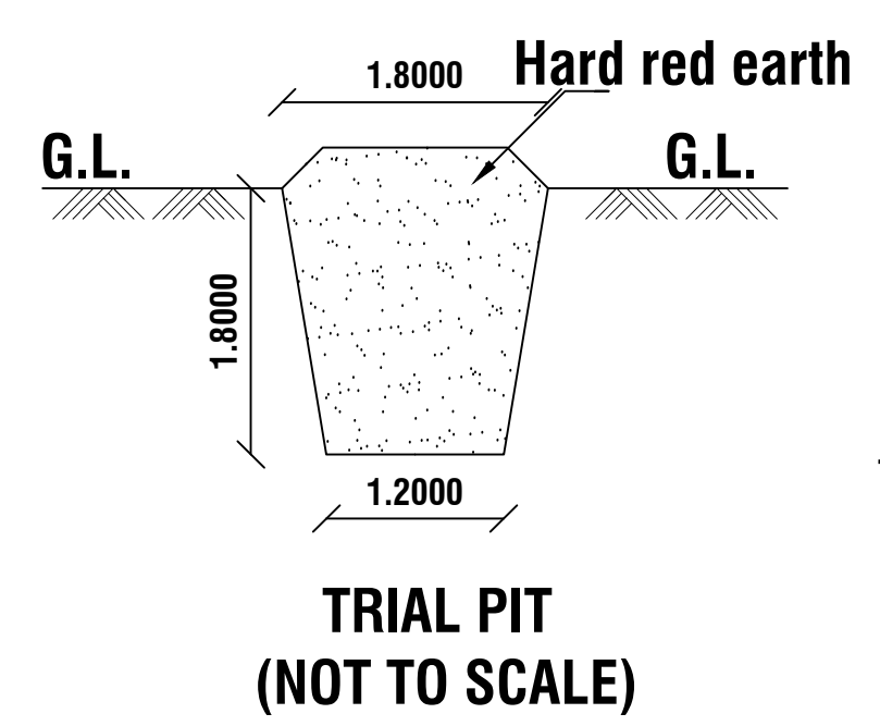
TRIAL PIT (NOT TO SCALE)
