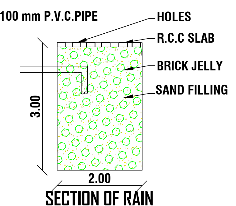
SECTION OF RAIN
