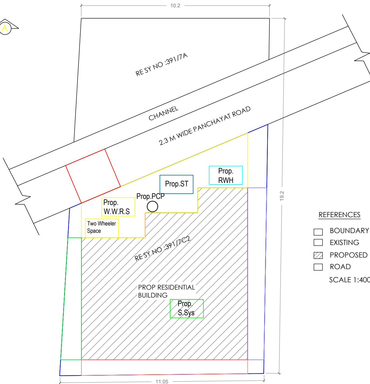
SITE PLAN
