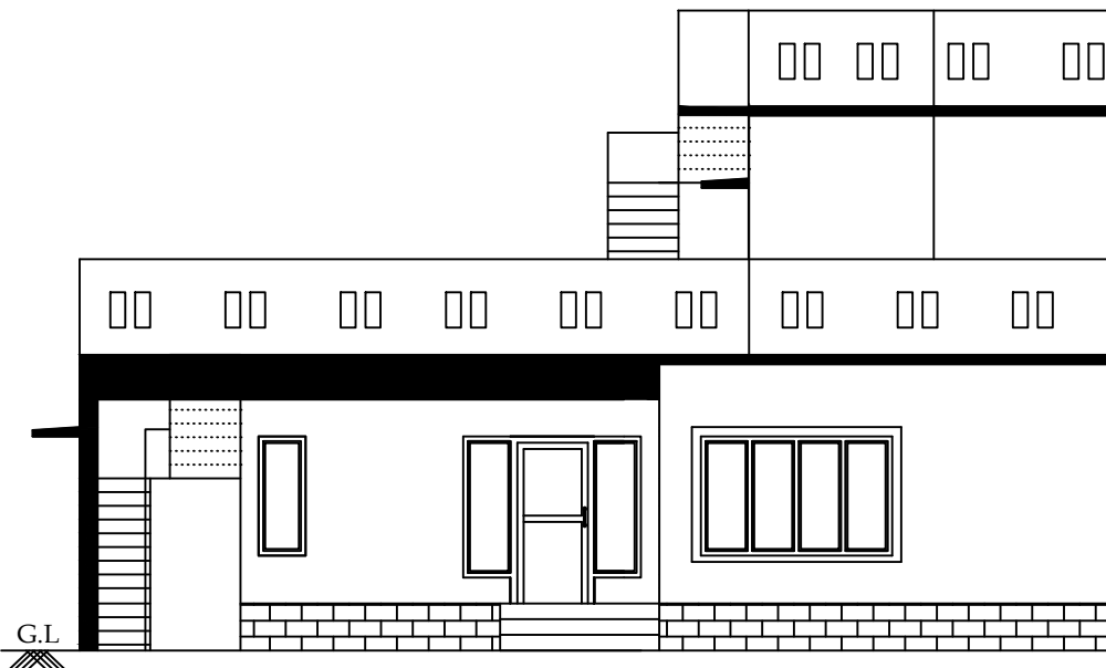
ELEVATION (SCALE 1:100)
