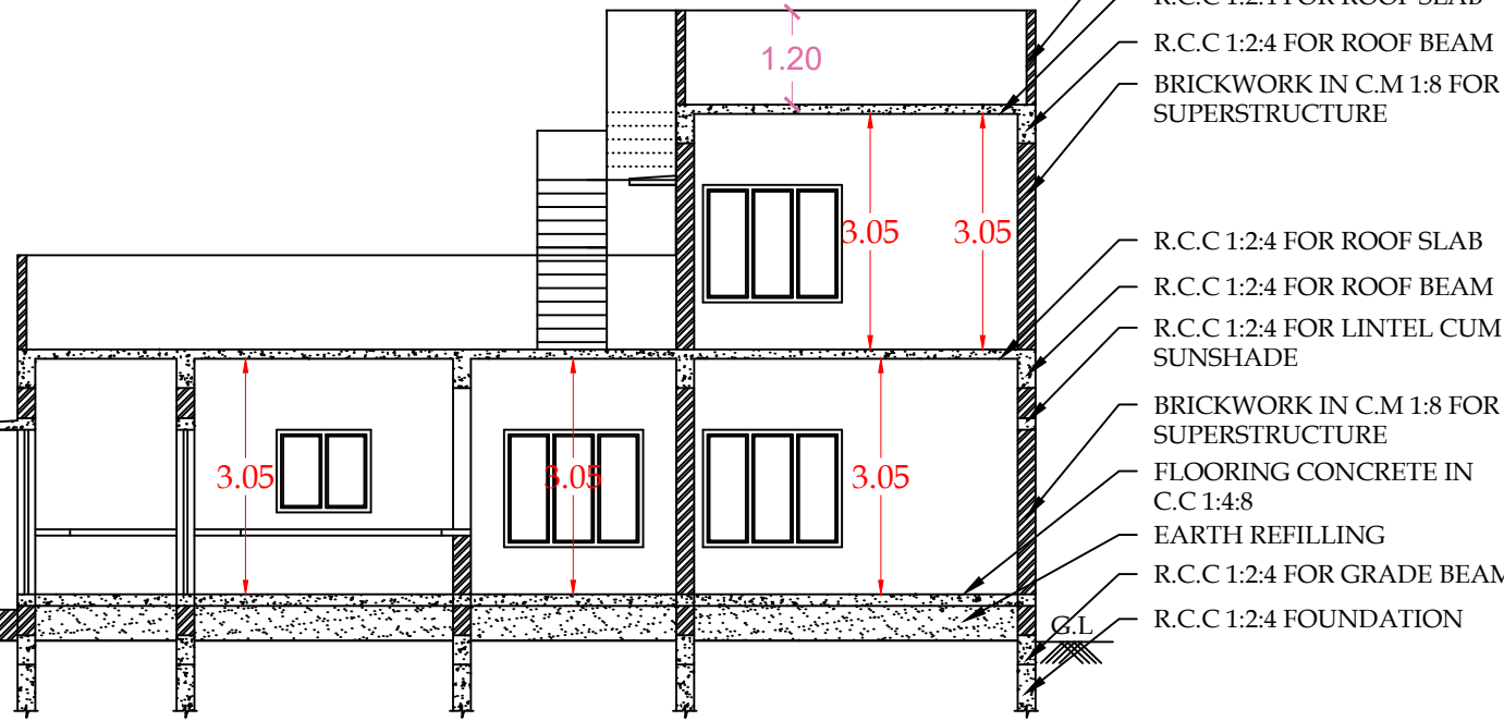
SECTION ON AB (SCALE 1:100)
