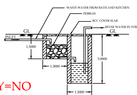
RE-CYCLING OF WASTE WATER FROM BATH AND KITCHEN
