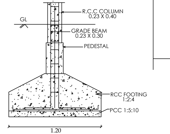
DETAILS OF COLUMN
