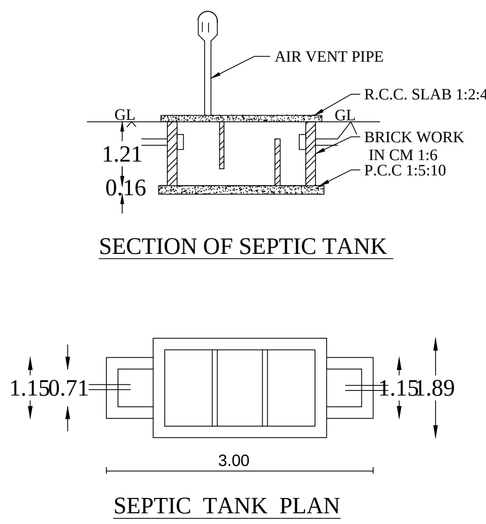
SEPTIC TANK PLAN
