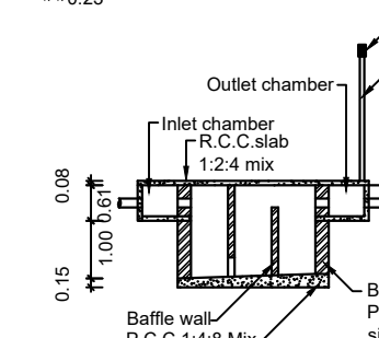
SECTION UV
