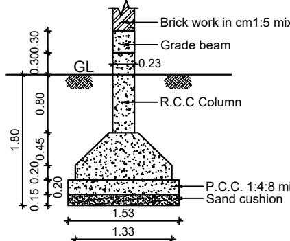
COLUMN DETAILS
