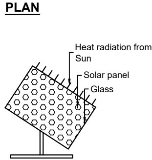
SOLAR SYSTEM
