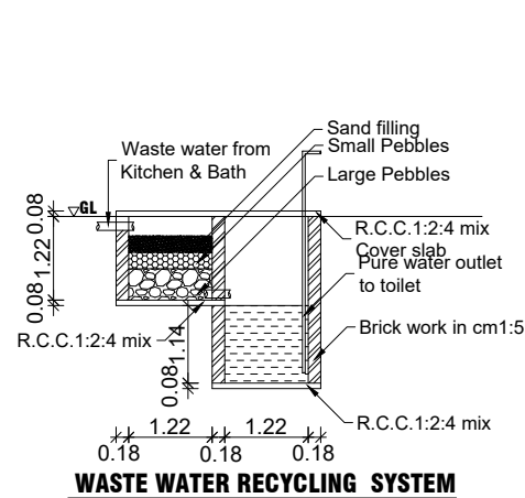
WASTE WATER RECYCLING SYSTEM
